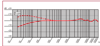
Top chart: Cardioid Bottom chart: Hypercardioid (with PPC 1000)
