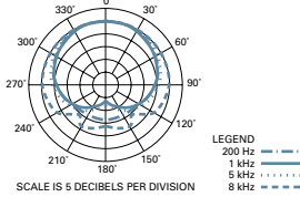
polar pattern
