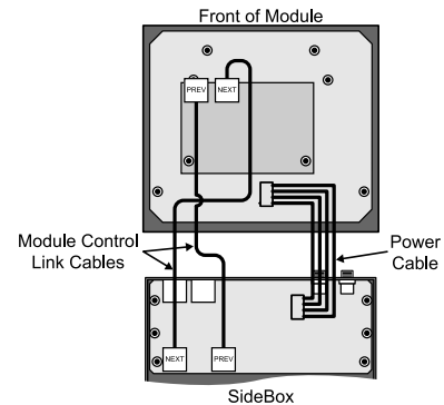
Figure 9: Disconnecting Internal Cables
