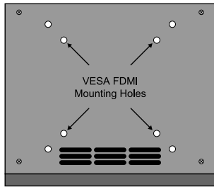
Figure 5: VESA Mounting Holes
