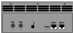
Figure 6: Cable Connections
