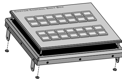
Figure 10: Removing Module
